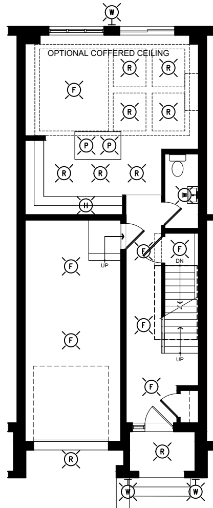
MAIN FLOOR LIGHTING LAYOUT
