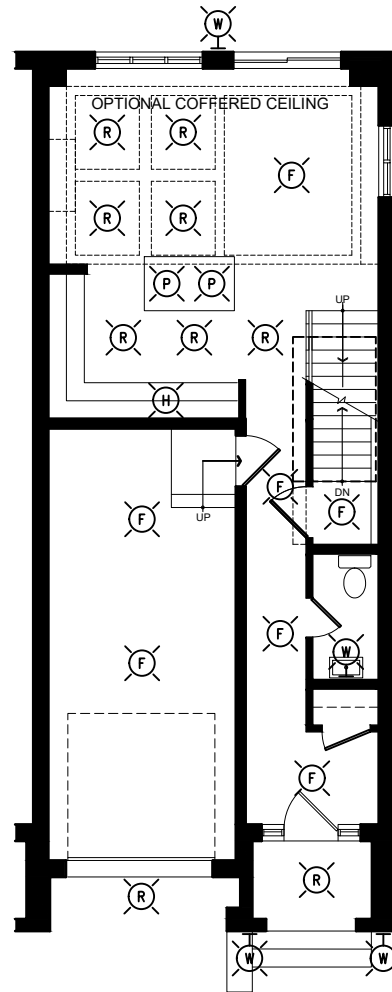
MAIN FLOOR LIGHTING PLAN
